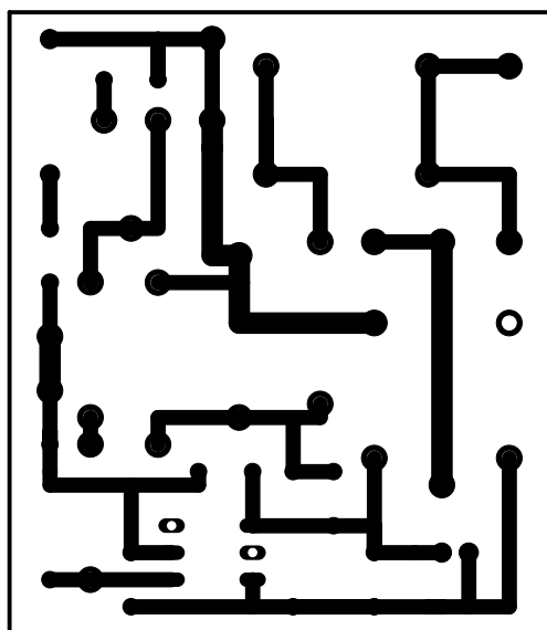
Z_BOT-MIRROR 50mm
